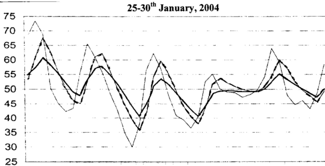
Figure 2a. Temperature data loggings during a cold period (25th to 30th of January 2004). The solid bold line represents adobe; the dashed line represents cinder block and the solid light line represents ambient temperature. Note that for every temperature extremes the cinder block had temperatures higher and lower than the adobe. Also fluctuation of temperature was greater for the cinder block than for the adobe.
